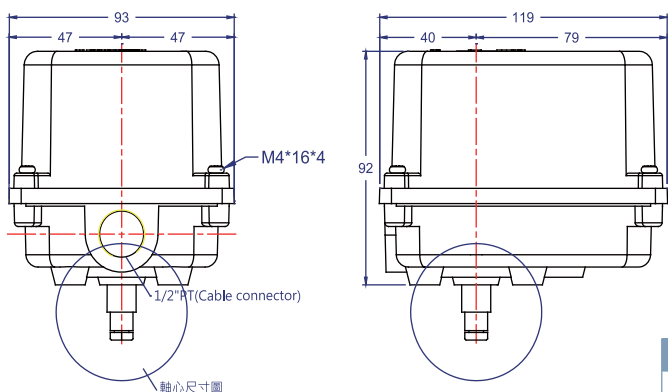
Mounting Flanged
