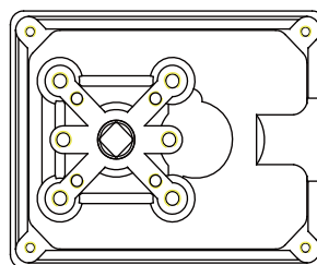
Mounting Flanged
